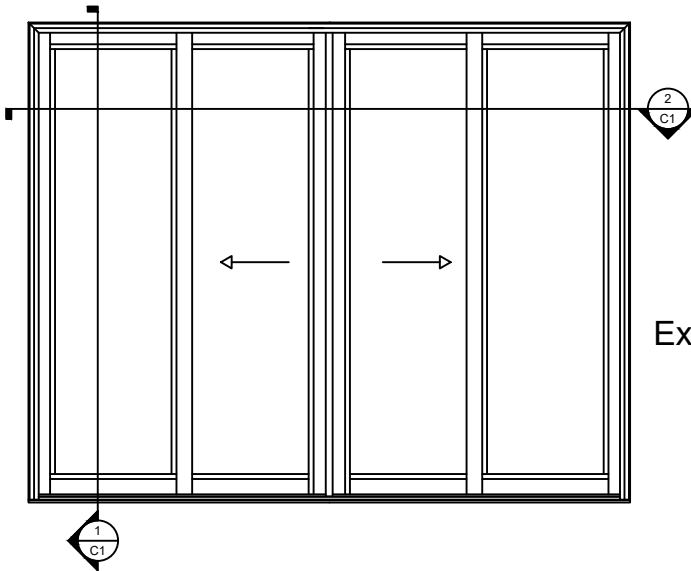
Window Elevation 3/8" = 1' 0"
